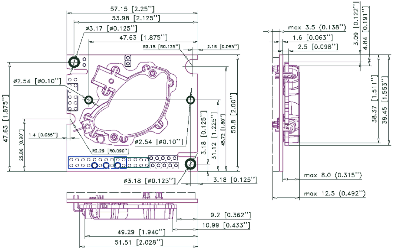
Figure 4. K30 mechanical drawing.
